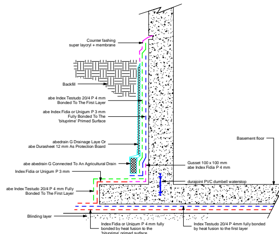
Typical Basement Detail Drawing 2
