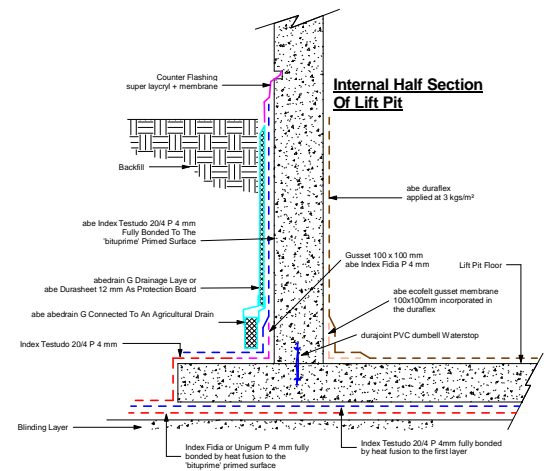
Typical Lift Pit Detail Drawing 3
