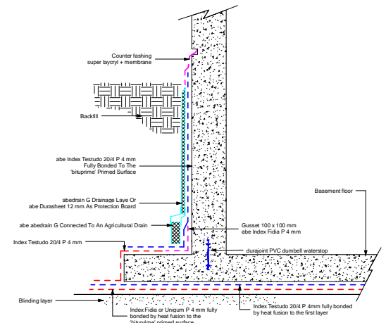
Typical Basement Detail Drawing 3
