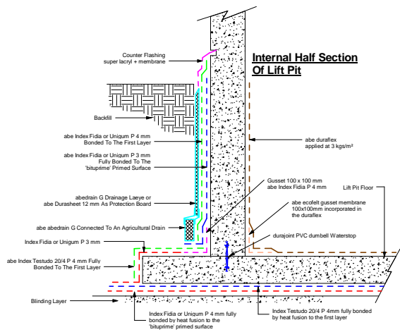
Typical Lift Pit Detail Drawing 1
