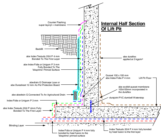
Typical Lift Pit Detail Drawing 2
