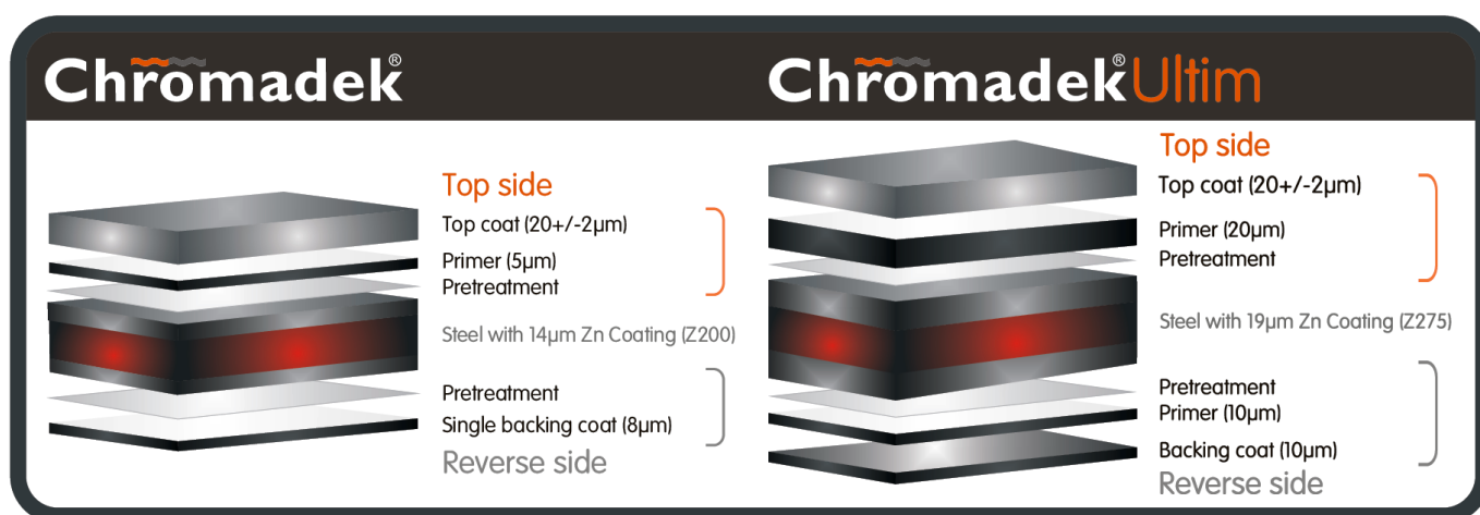
Figure 1: Coating structure of Chromadek® Standard and Chromadek Ultim®.
