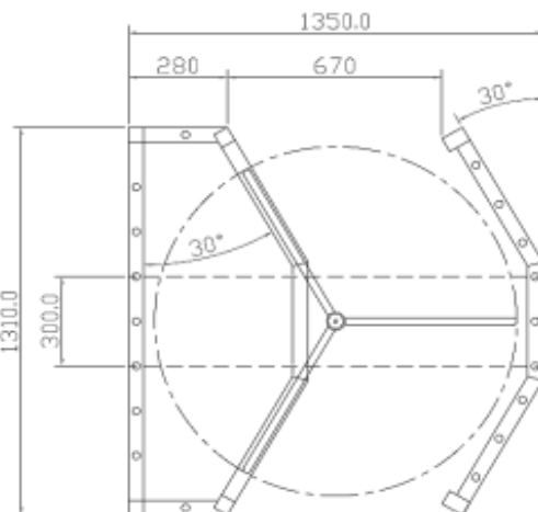
3-ARM SINGLE TURNSTILE
