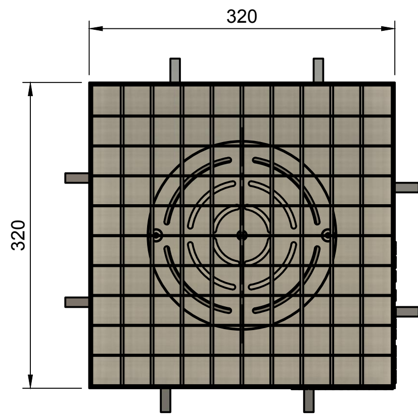
Top View Scale 1:4
