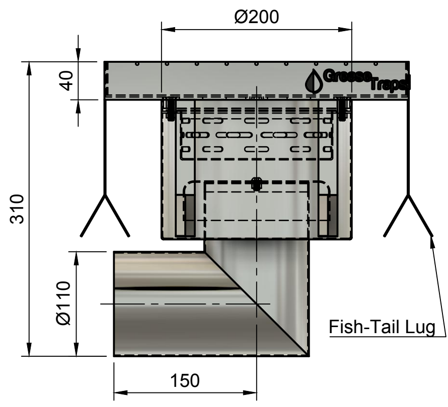
Front View Scale 1:4
