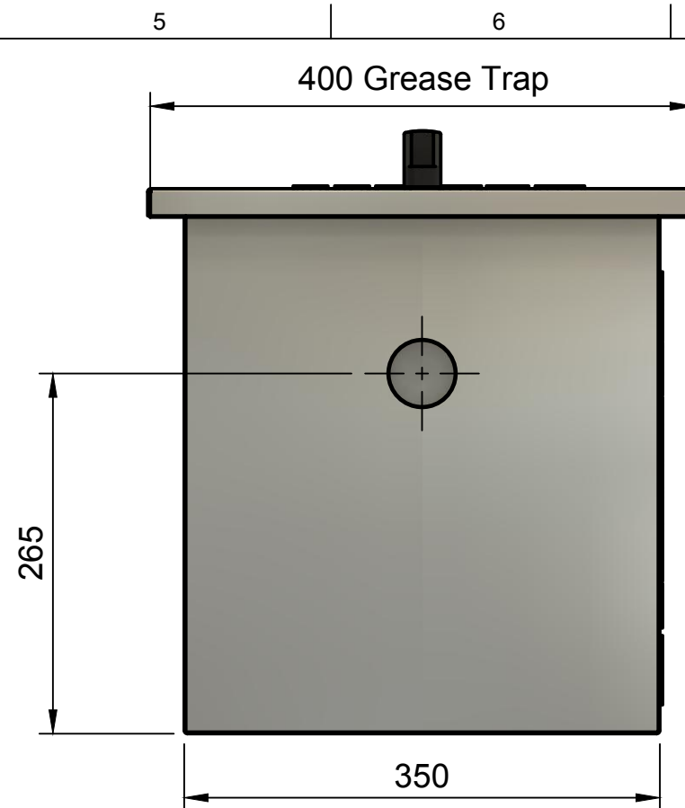
Front View Scale 1:5
