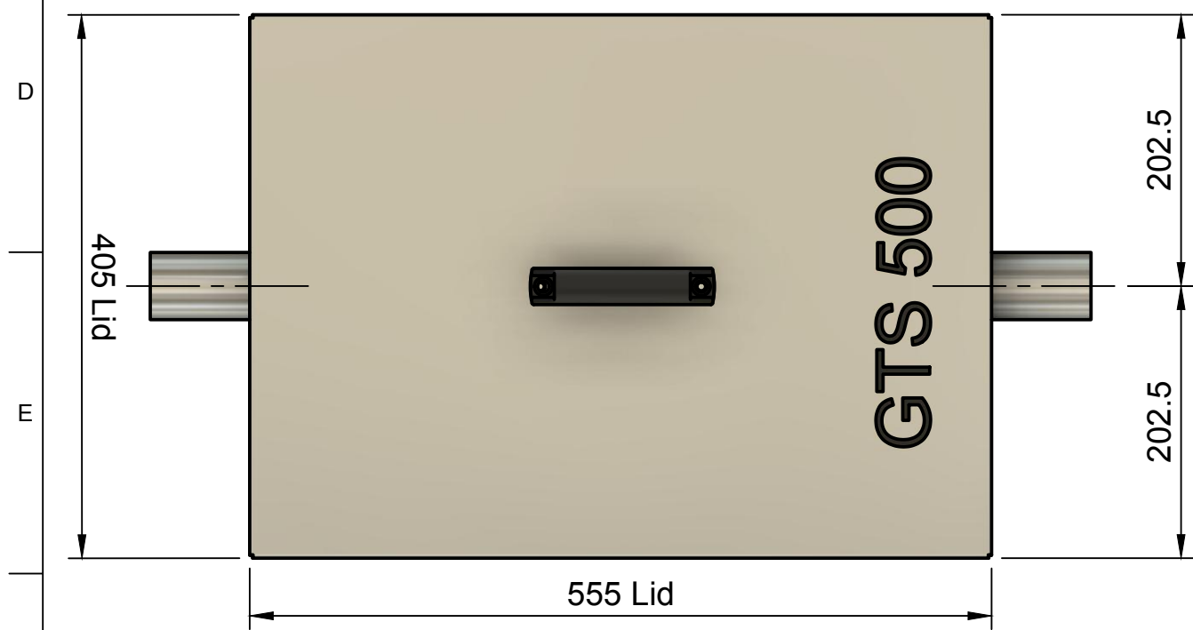
Top View Scale 1:5
