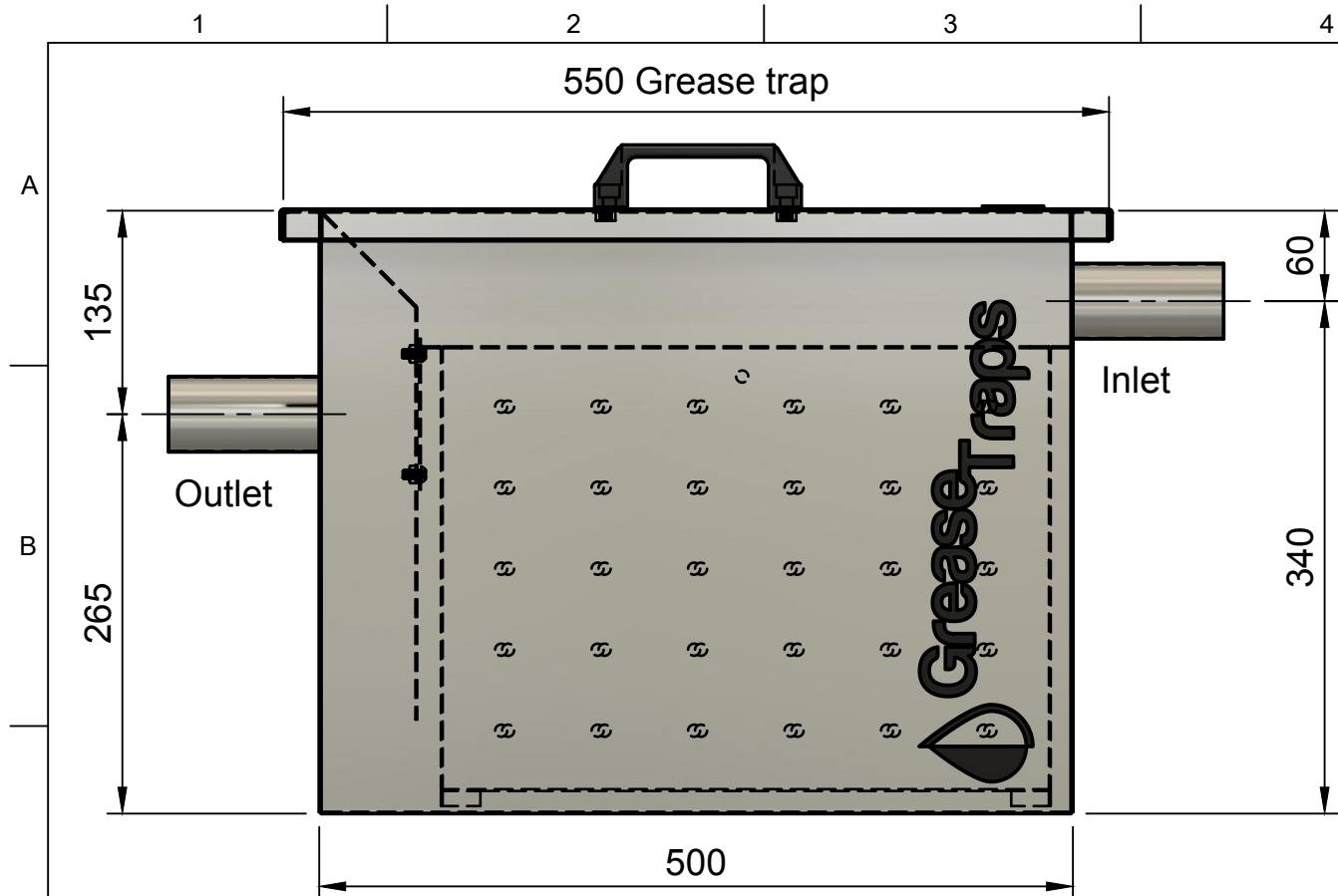
Side View Scale 1:5
