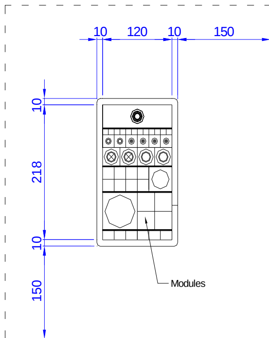
Multi Cable Transit Type SS / SSF-6x1
