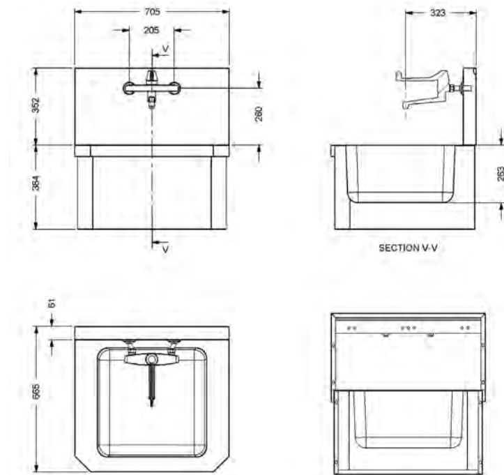
SBS Shown with optional Cobra 508 Medical Mixer
