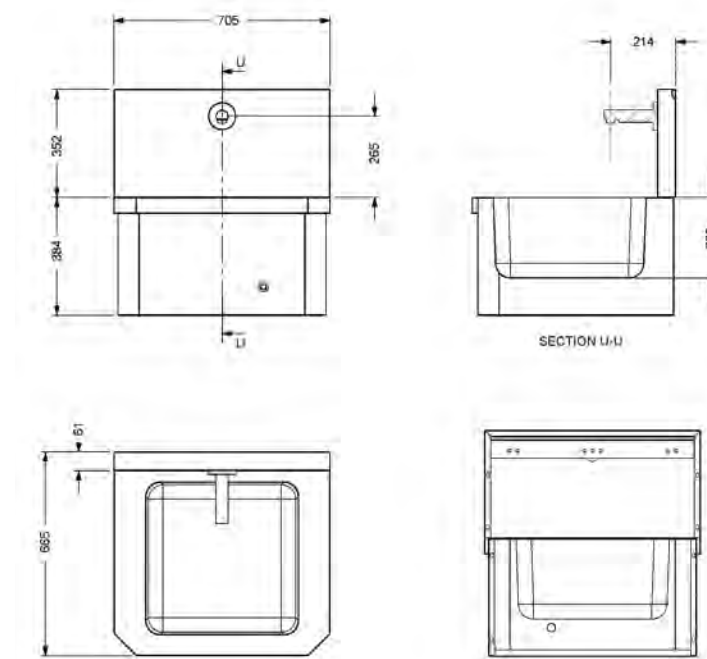
Sensor Operated Scrub SBSS
