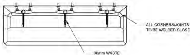
SB Elbow Action Scrub Unit
