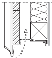
Dia. 20.1: Base flush, with ventilation
