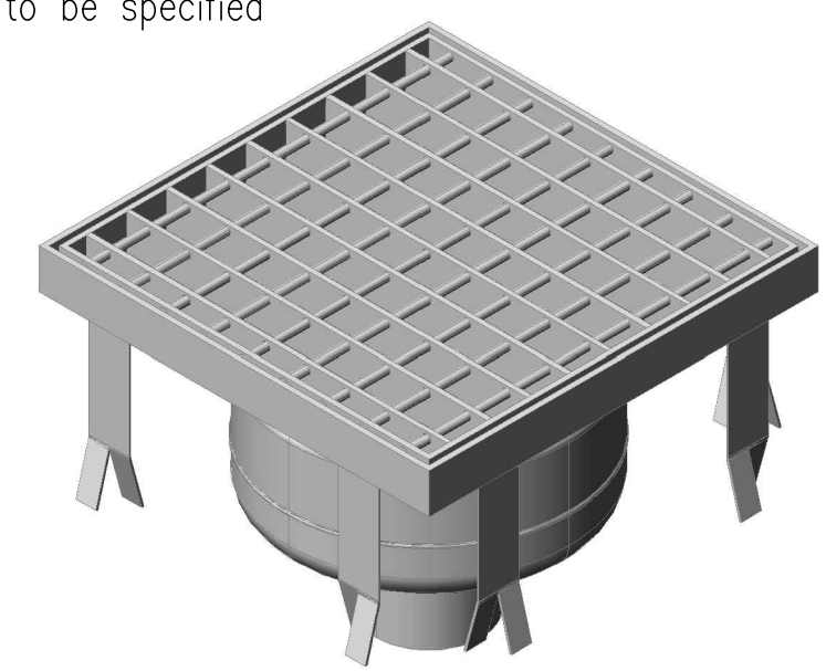
RO 280V NW100 HEAVY DUTY WITH GRATING
