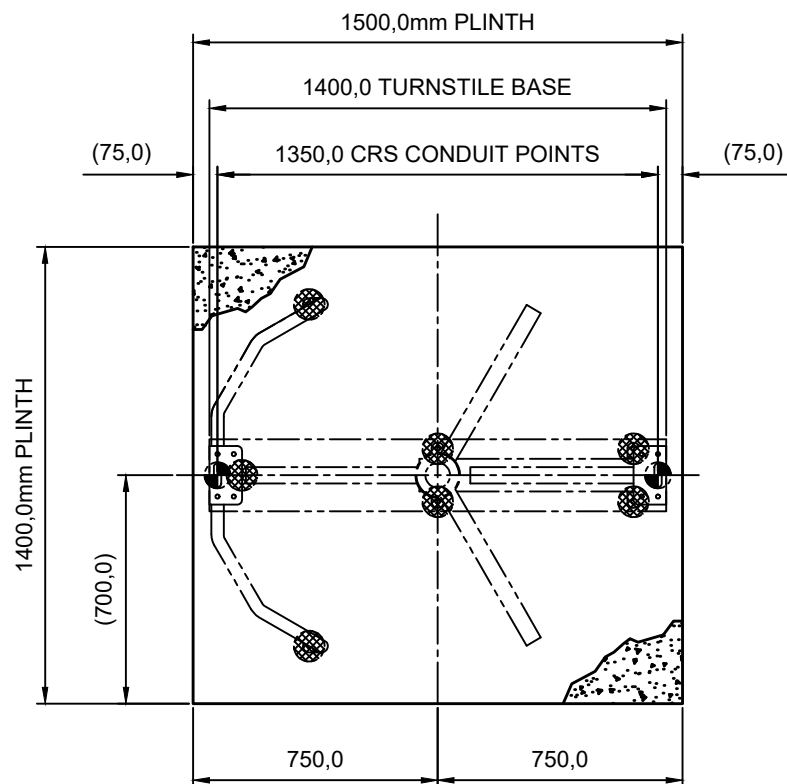
PLAN VIEW (TURNSTILE IN REF. LINE)
