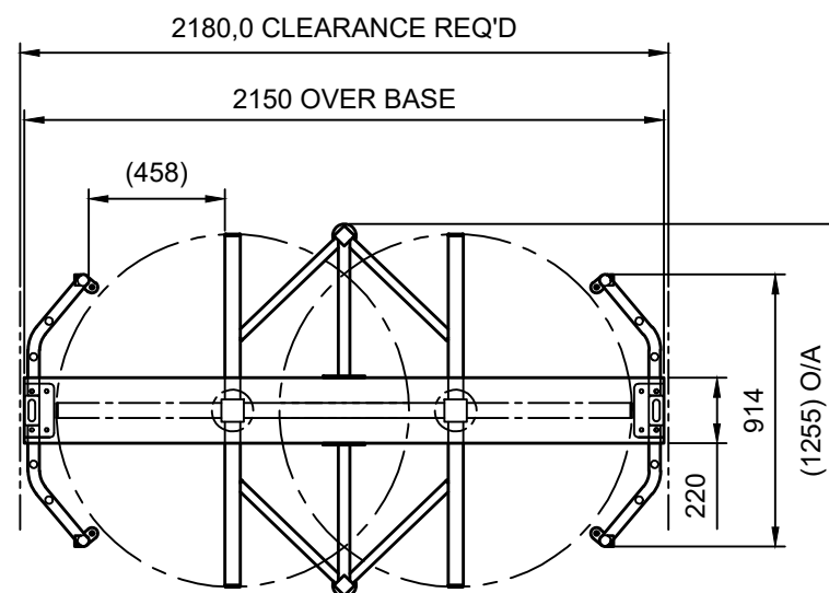
PLAN (COVER OMITTED)
