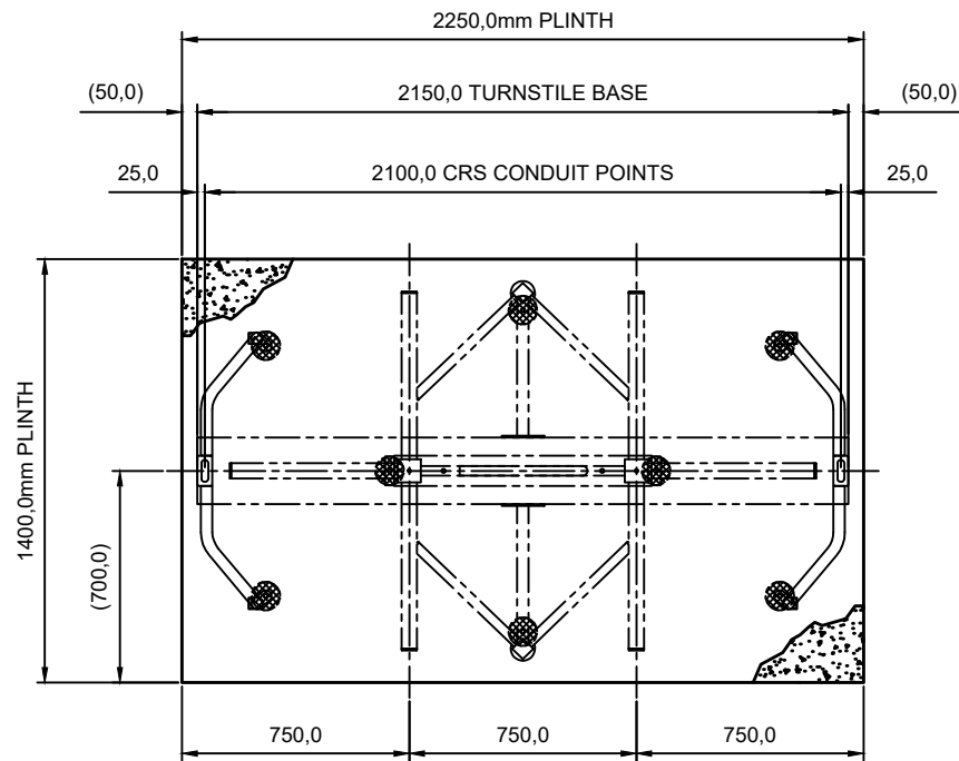
PLAN VIEW (TURNSTILE IN REF. LINE)
