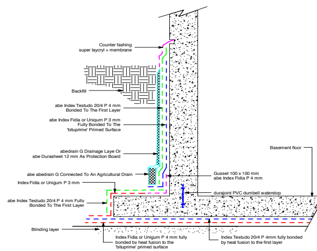
Typical Basement Detail Drawing 2
