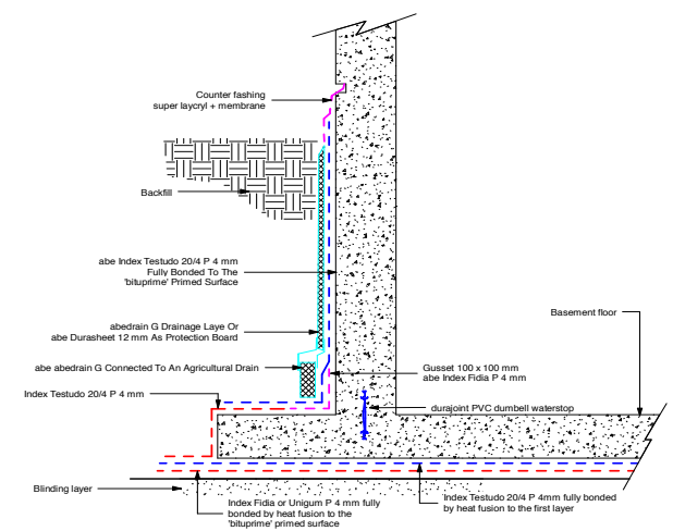
Typical Basement Detail Drawing 3
