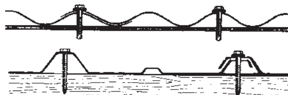
IBR to timber support
