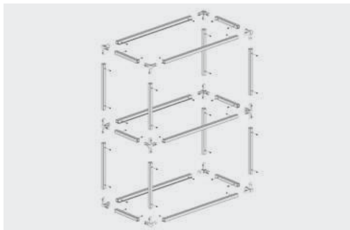
Top cabinet vCUBE frame: for 3 timber shelves on the top, bottom and middle
