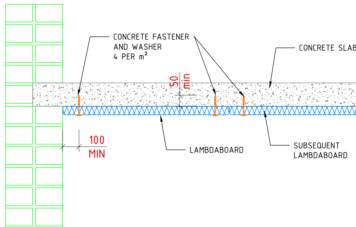
SECTION VIEW ON UNDER SOFFIT APPLICATION N.T.S.
