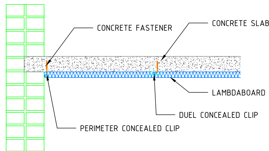
SECTION VIEW ON UNDER SOFFIT APPLICATION N.T.S.
