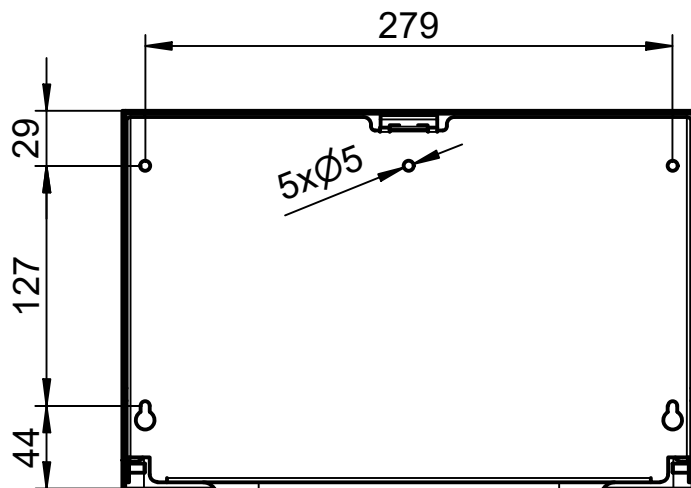
Bohrbild | drilling pattern
