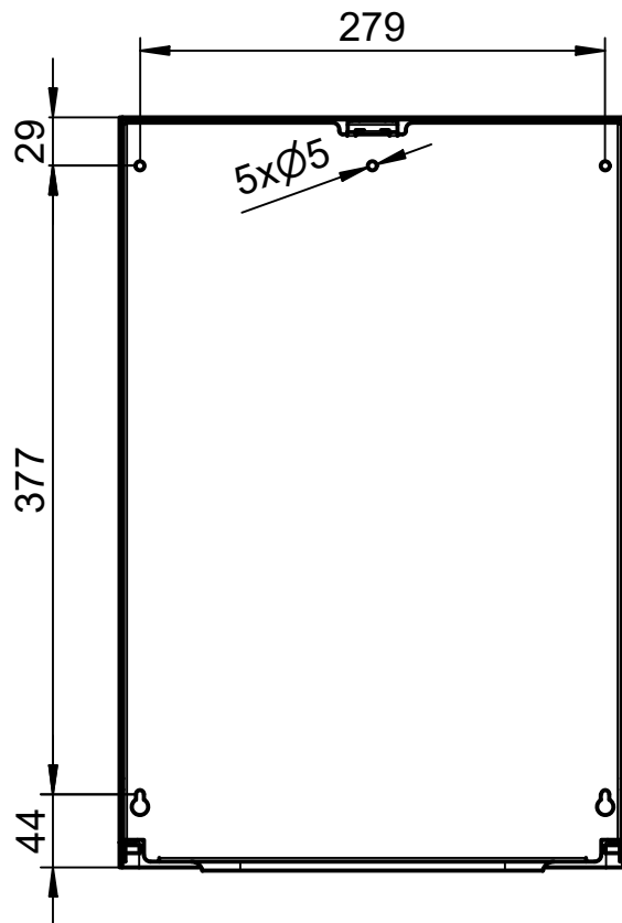
Bohrbild | drilling pattern
