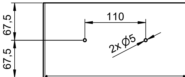
Bohrbild | drilling pattern
