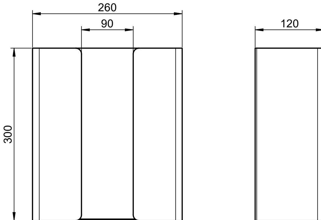
Bohrbild | drilling pattern
