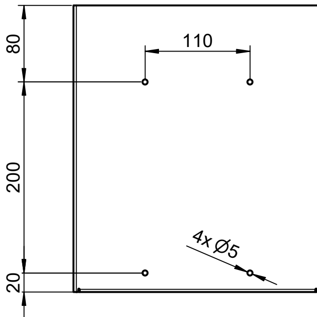
Bohrbild | drilling pattern
