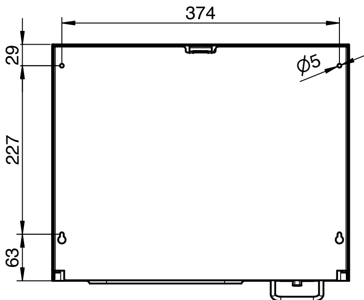
Bohrbild I drilling pattern
