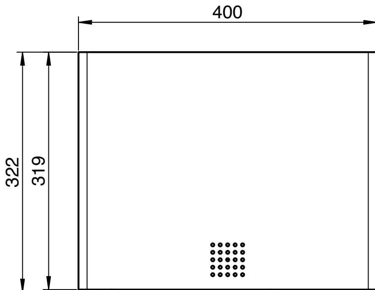
Bohrbild I drilling pattern
