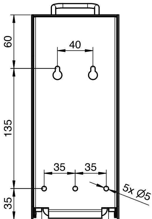
Bohrbild I drilling pattern
