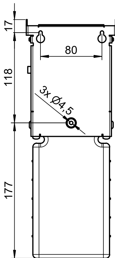
Bohrbild | drilling pattern
