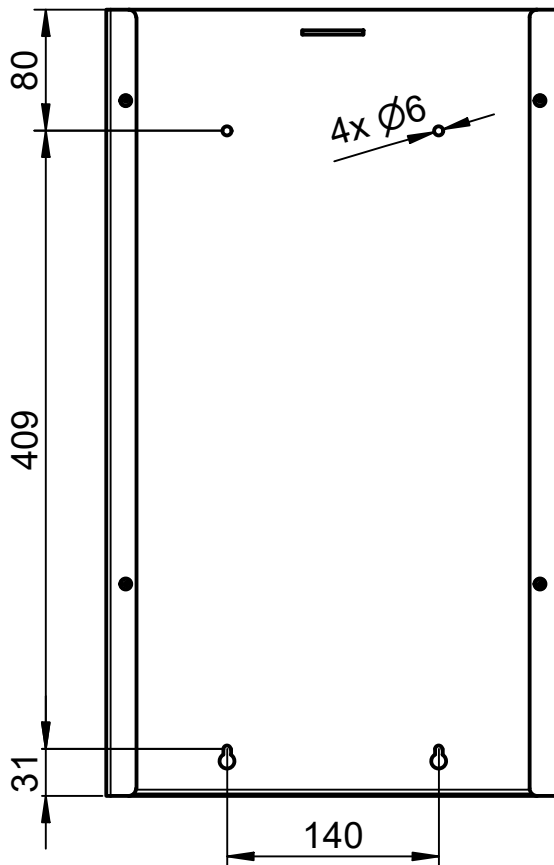
Bohrbild | drilling pattern
