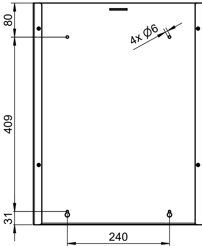
Bohrbild | drilling pattern
