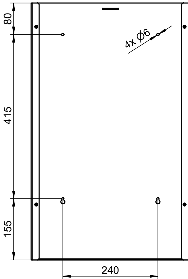
Bohrbild | drilling pattern
