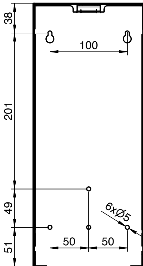
Bohrbild I drilling pattern
