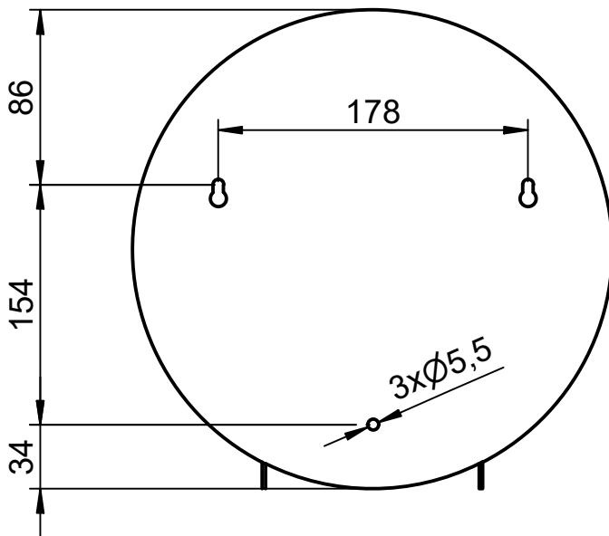
Bohrbild | drilling pattern
