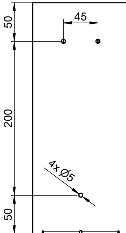
Bohrbild | drilling pattern
