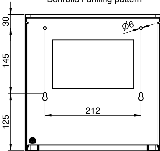
Bohrbild I drilling pattern
