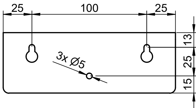
Bohrbild | drilling pattern
