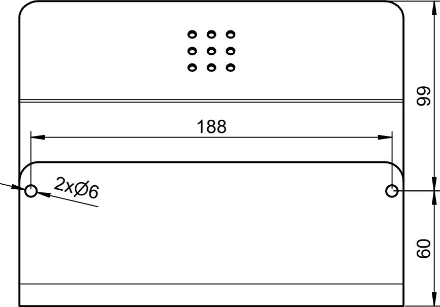
Bohrbild | drilling pattern
