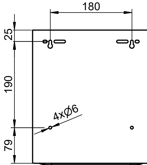
Bohrbild | drilling pattern
