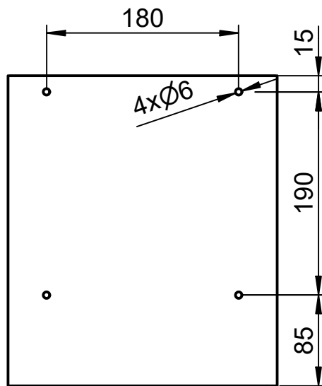
Bohrbild | drilling pattern
