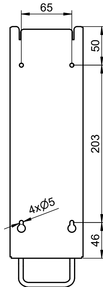
Bohrbild | drilling pattern
