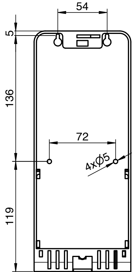
Bohrbild I drilling pattern
