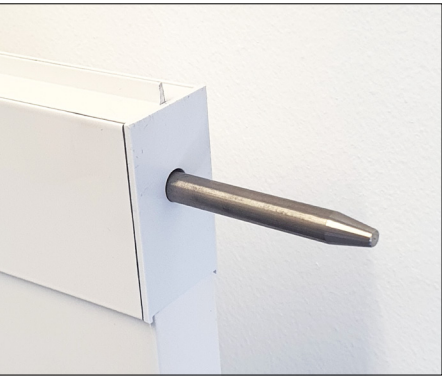
60 mm patented bolt secures shutters to floor when locked
