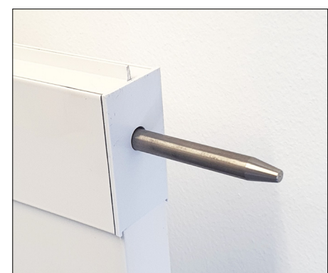
60 mm patented bolt secures shutters to floor when locked
